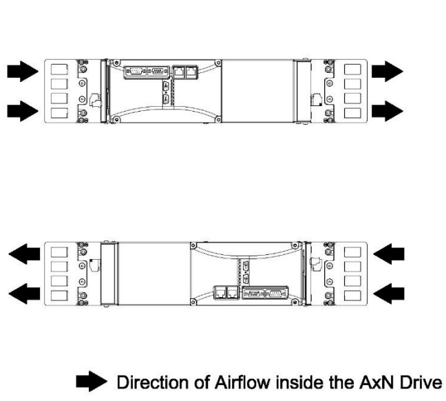
Installation Orientation of AxN Size2 Series Drive
