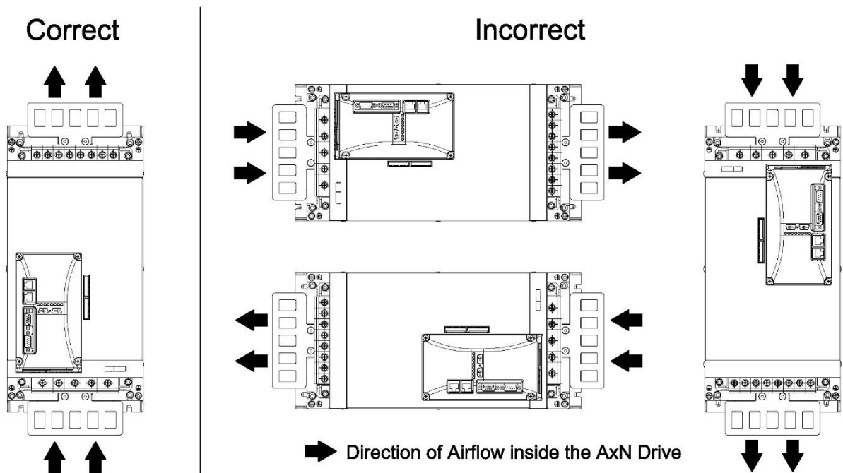
Installation Orientation of AxN Size4 Series Drive
