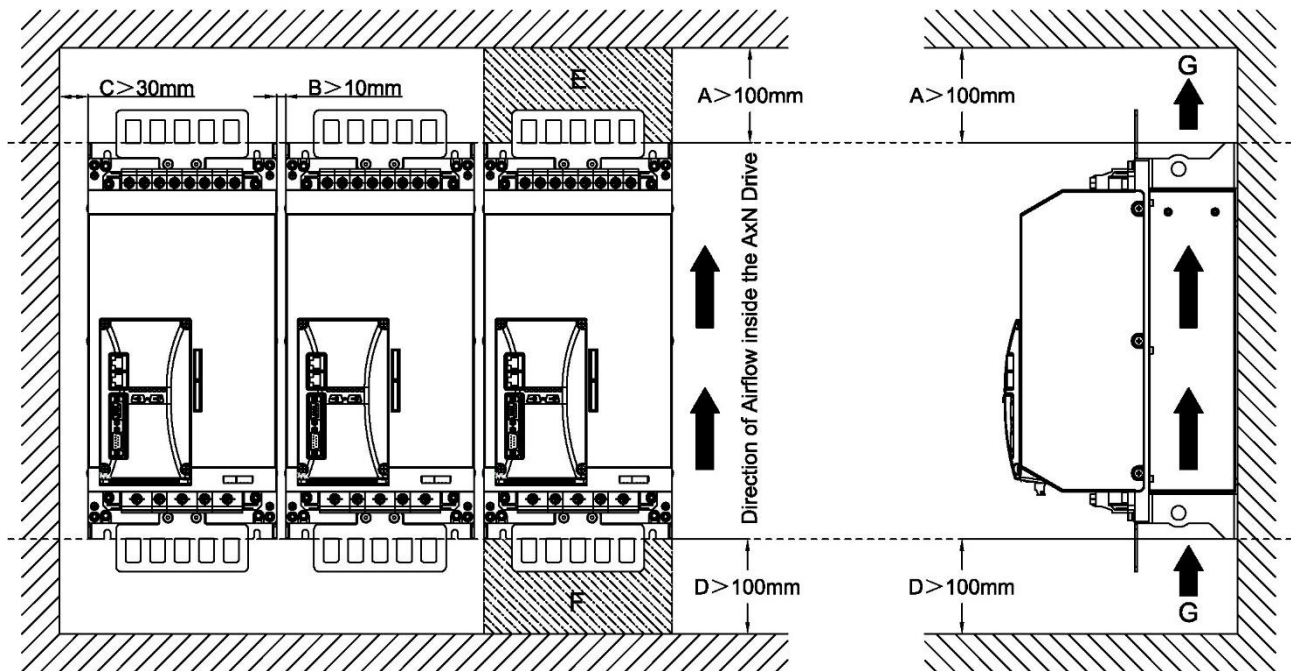
Installation Spacing of AxN Size4 Series Drive
