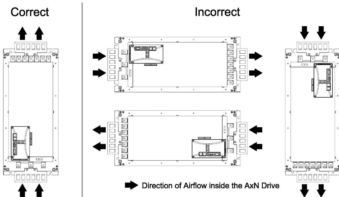
Installation Orientation of AxN Size5 Series Drive
